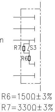
Wiring diagram
